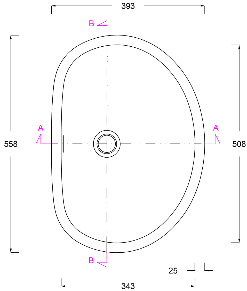
PLAN VIEW
